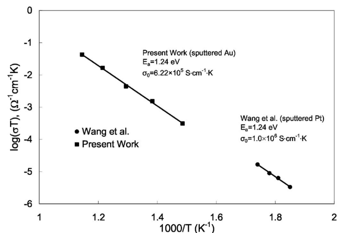
Figure 4. Arrhenius plot of the total conductivity of \text{Li}_3\text{PO}_4 electrolyte with gold-ion-blocking electrode.
