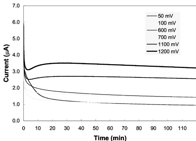
Figure 8. A typical time response of the current in Hebb-Wagner measurement for \text{Li}_3\text{PO}_4 at 500^\circ\text{C} .
