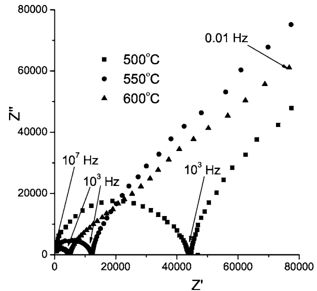
Figure 3. Impedance plot of gold-ion-blocking electrode for \text{Li}_3\text{PO}_4 at 500, 550, and 600^\circ\text{C} .
