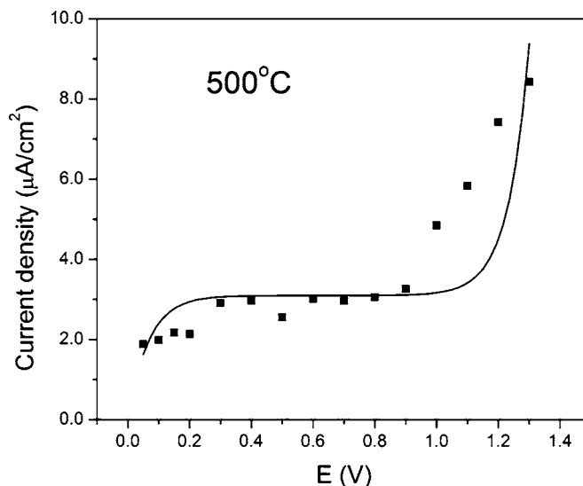
Figure 9. Hebb-Wagner polarization curve for \text{Li}_3\text{PO}_4 ; steady-state current as a function of the applied voltage at 500^\circ\text{C} .
