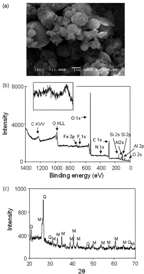
Figure 4. Characteristics of the CFA particles: (a) SEM, (b) XPS (inset is the iron region, with the peaks due to Fe 3+ marked), and (c) powder X-ray diffraction (Q = quartz; M = mullite).
