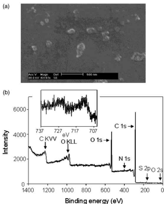
Figure 5. Characteristics of the DEP: (a) SEM and (b) XPS (inset is the iron region, with the peaks due to Fe 3+ marked). exposed M \phi s upon proximal endothelia, human ECs derived from umbilical vein (hUVEC), pulmonary artery
