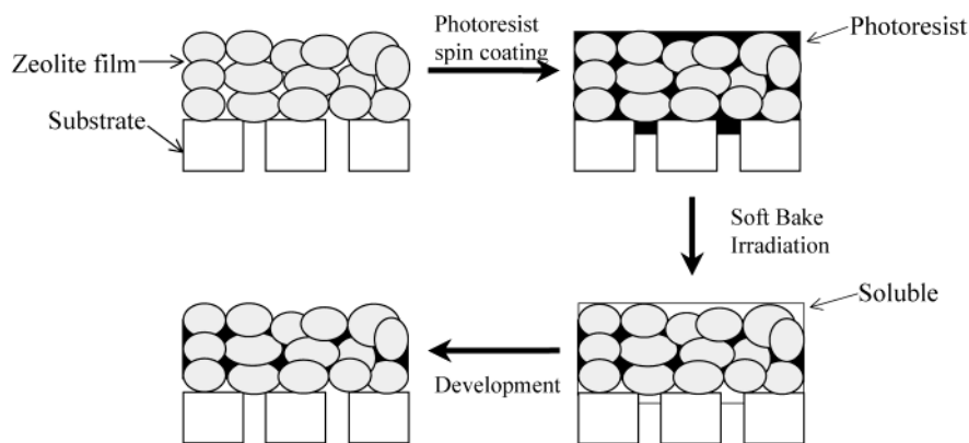
Figure 7. Photoresist coating process.
