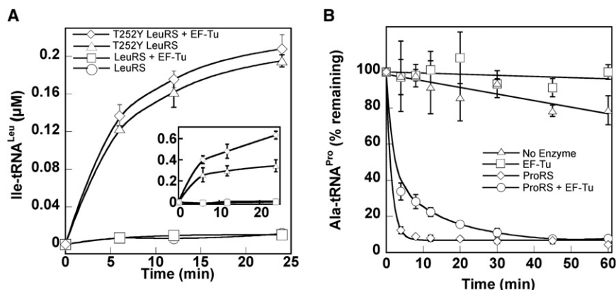
Figure 3. Misacylation by LeuRS and ProRS
