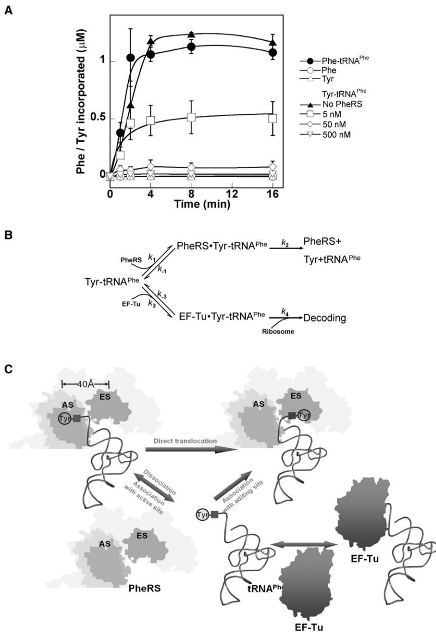
Figure 4. Resampling and Editing of Mischarged tRNA
