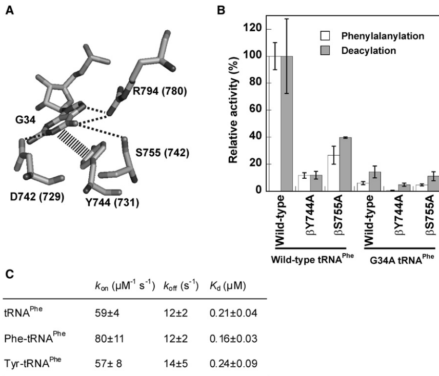
Figure 2. Recognition of E. coli tRNA Phe during Aminoacylation and Editing
