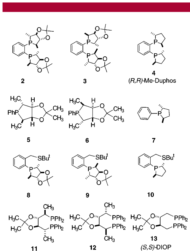
Figure 1. Functionalized phospholanes and phosphines for Pd(0)-catalyzed allylation.
