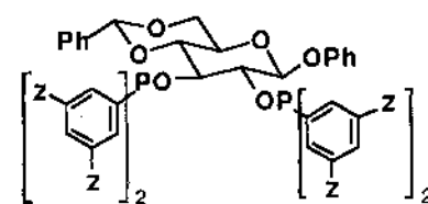
Fig. 2. Structure of the diol phosphinite ligand L* in Eq. 1. Ph, phenyl.
